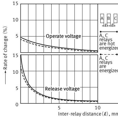
5-1. Influence of proximity mounting ( 1 Form A )
