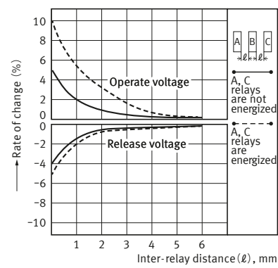
5-2. Influence of proximity mounting ( 1 Form A 1 Form B )
