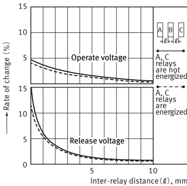
5-3. Influence of proximity mounting ( 2 Form A )
