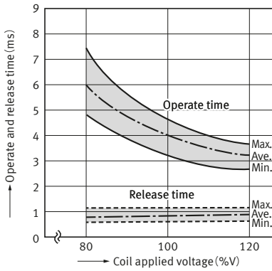
4-3. Operate and release time ( without diode: 2 Form A )
