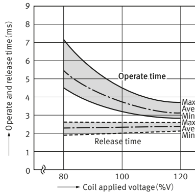
4-4. Operate and release time ( with diode: 1 Form A )
