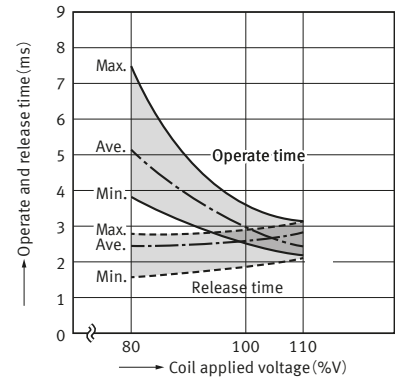
4-5. Operate and release time ( with diode: 1 Form A 1 Form B )
