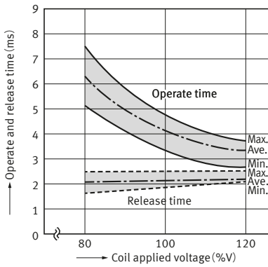
4-6. Operate and release time ( with diode: 2 Form A )
