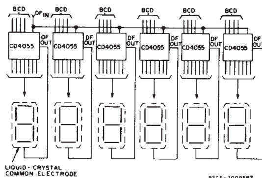
Fig. 16 - Clock display: V_{DD} = 0 V, V_{SS} = -5 V, V_{EE} = -15 V, DF_{IN} = 30 Hz square wave.
