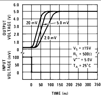
Figure 17. Response Time for Various Input Overdrives
