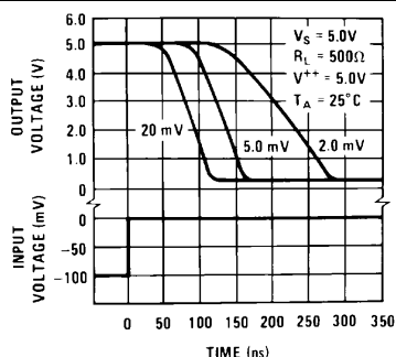
Figure 19. Response Time for Various Input Overdrives
