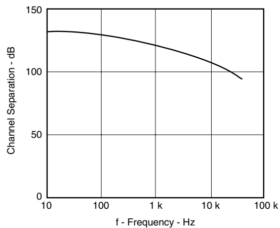
CHANNEL SEPARATION
